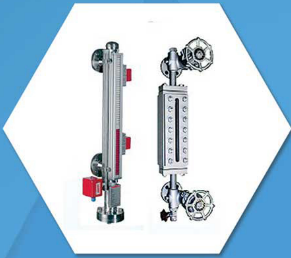
Magnetic , Reflex, Transparent & Float & Board Type Level Gauges
